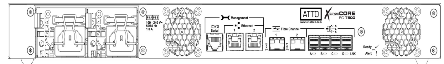
Exhibit 2 XstreamCORE™ FC 7500, LEDs, power receptacle and ports
