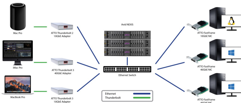
Workgroup configuration with ATTO ThunderLink 40GbE and 10GbE Thunderbolt adapters and FastFrame NICs connecting both desktop and mobile workstations to Avid NEXIS storage
