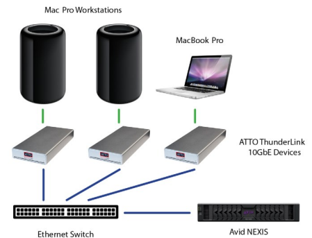
Workgroup configuration with ATTO ThunderLink 10GbE Thunderbolt devices and FastFrame NICs connecting Mac Pro desktop and mobile workstations to Avid NEXIS
