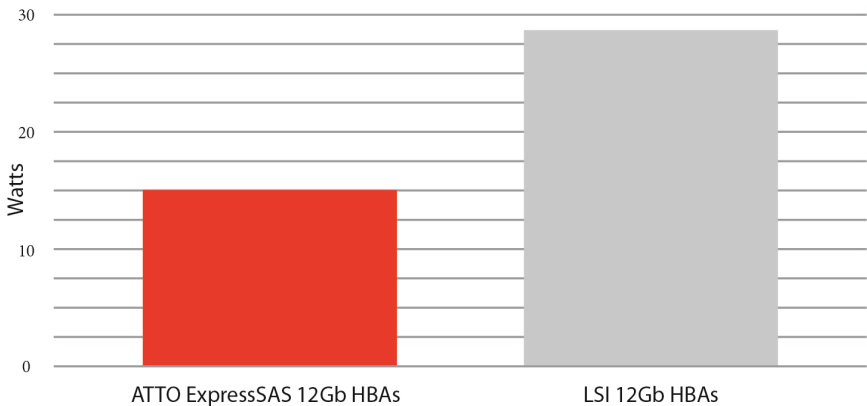
Comparing ATTO ExpressSAS 12Gb HBA to LSI 16-port HBA. ATTO draws 15 watts versus LSI at 28.6 watts – 48% less.
