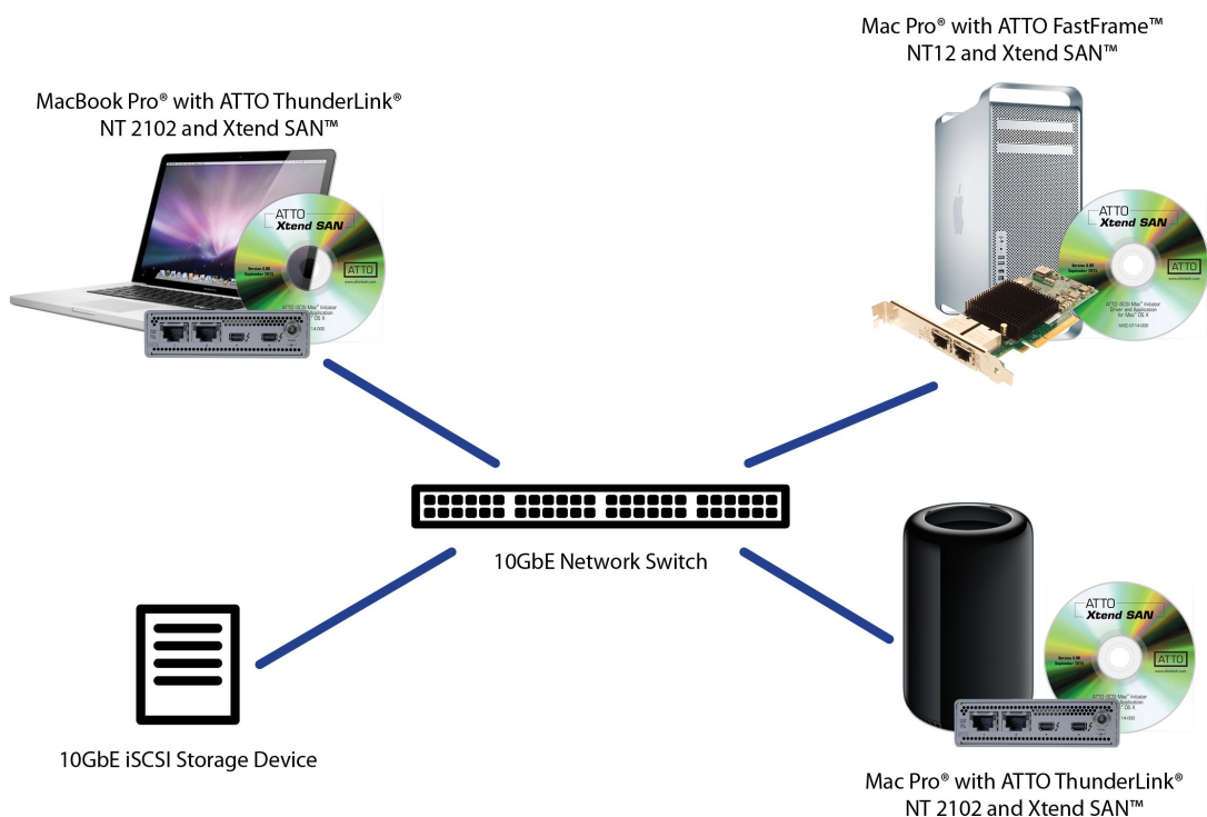
Fig. 1: Example of iSCSI Digital Video SAN
