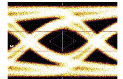
Substandard Cable Signal: Distorted eye pattern = weaker signal integrity Possible data loss, errors
