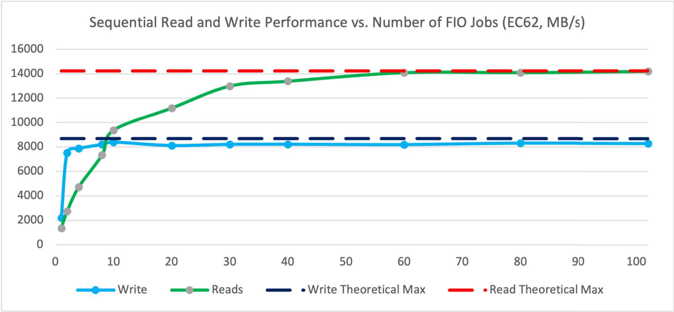
Fig 2: Read-Write performance achieved with Leil's SMR optimization
